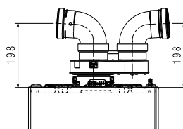
Ø80-80 mm TWIN FLUE with ADAPTER
