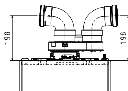
TWIN FLUE Ø80-80 mm WITH ADAPTER
