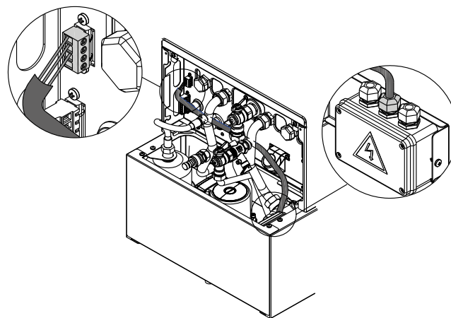
Connect the BUS 485 signal cable
