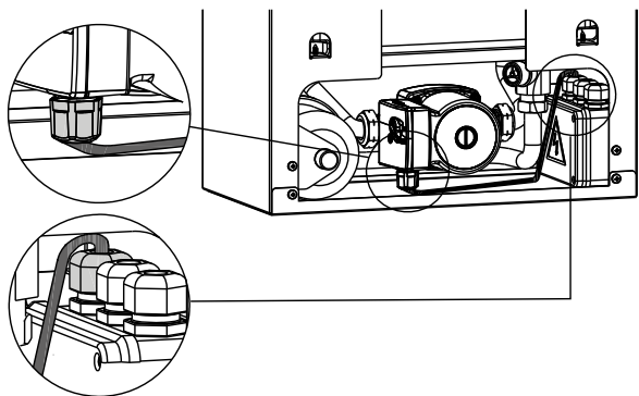
Remove the 4-way connector located under the boiler shelf
