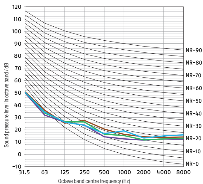
Cooling A35W7
